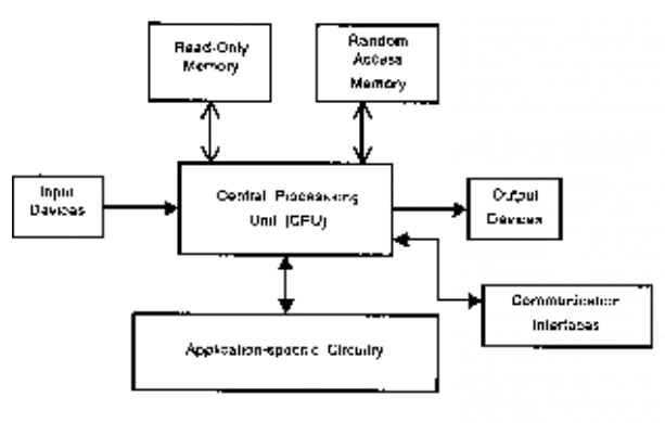
Fig: 3.1 Building blocks of the hardware of an embedded system
